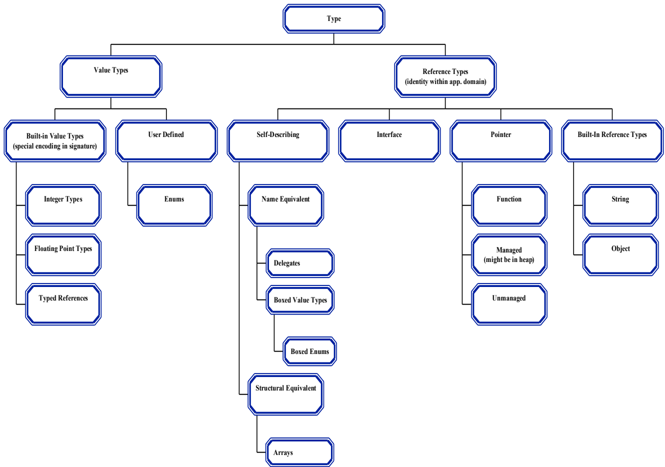
Figure 1: Type System
